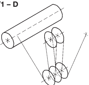
Type 6/1 – D
