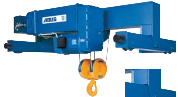
Articulated end carriage joint
