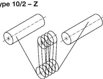
Type 10/2 – Z
